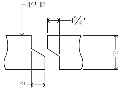
TONGUE AND GROOVE DETAIL
