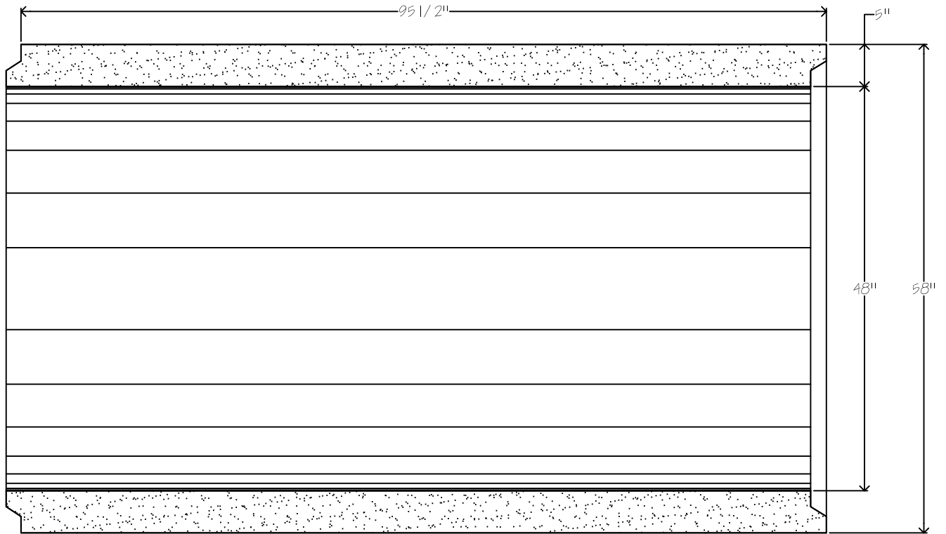
48" RCP PIPE DETAIL
