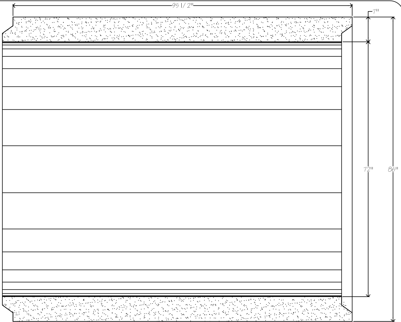
72" RCP PIPE DETAIL
