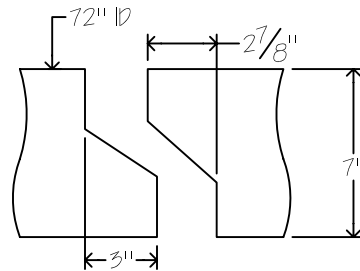
72" RCP PIPE DETAIL
